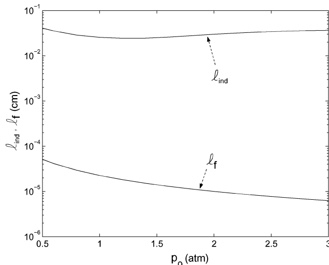
Fig. 5 Induction zone length and finest length scale vs initial pressure.
